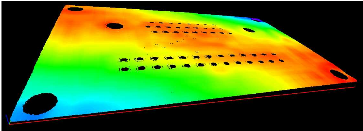
Warpage = 0.145 mm
